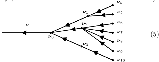
Fig. 5: An example of a tree graph and of its labels. It contains only one simple node (3). Harmonics are indicated next to their nodes. Labels distinguishing lines are not marked.
