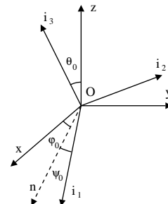
Fig. 3: The Euler angles of the comoving frame \mathbf{i}_1, \mathbf{i}_2, \mathbf{i}_3 with respect to a fixed frame \mathbf{x}, \mathbf{y}, \mathbf{z} . The direction \mathbf{n} is the “node line, intersection between the planes \mathbf{x}, \mathbf{y} and \mathbf{i}_1, \mathbf{i}_2 .”
