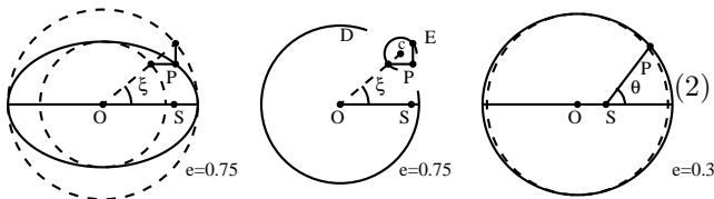
Fig. 2: Eccentric and true anomalies of P which moves on a small circle E centered at a point c moving on the circle D located half way between the two concentric circles containing the Keplerian ellipse: the anomaly of c with respect to the axis OS is \xi . The circle D is eccentric with respect to S and therefore \xi is, still today, called eccentric anomaly while the circle D is, in ancient terminology, the deferent circle (eccentric circles were introduced in Astronomy by Ptolemy). The small circle E on which the point P moves is, in ancient terminology, an epicycle . The deferent and the epicyclical motions are synchronous (i.e. have the same period); Kepler discovered that his key a priori hypothesis of inverse proportionality between angular velocity on the deferent and distance between P and S (i.e. \rho\dot{\xi} = \text{constant} ) implied both synchrony and elliptical shape of the orbit, with focus in S . The latter law is equivalent to \rho^2\dot{\theta} = \text{constant} (because of the identity a\dot{\xi} = \rho\dot{\theta} ). Small eccentricity ellipses can be hardly distinguished from circles.
