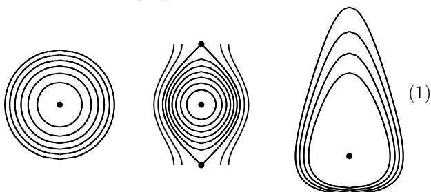
Fig. 1: The energy levels of the harmonic oscillator, the pendulum, and the Kepler motion
