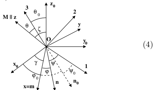
Fig. 4: The laboratory frame, the angular momentum frame, the comoving frame (and the Deprit angles).
