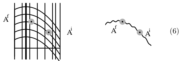
Fig. 6: The first drawing represents the \varepsilon = 0 geometry: the “partial energy” lines are parabolae, \frac{1}{2}A_1^2 + A_2 = \text{const} . The vertical lines are the resonances A_1 = \text{rational} (i.e. \nu_1 A_1 + \nu_2 = 0 ). The disks are neighborhoods of the points \mathbf{A}^i and \mathbf{A}^f (the dots at their centers). The second drawing ( \varepsilon \neq 0 ) is an artist rendering of a trajectory in \mathbf{A} space, driven by the pendulum swings to accelerate the wheel from A_1^i to A_1^f at the expenses of the clock energy, sneaking through invariant tori not represented and (approximately) located “away” from the intersections between resonances and partial energy lines (a dense set, however). The pendulum coordinates are not shown: its energy stays close to 0 within a power of \varepsilon . Hence the pendulum swings staying close to the separatrix. The oscillations symbolize the wiggly behavior of the partial energy \frac{1}{2}A_1^2 + A_2 in the process of sneaking between invariant tori which, because of their invariance, would be impossible without the pendulum. The energy \frac{1}{2}A_1^2 of the wheel increases slightly at each pendulum swing: accurate estimates yield an increase of the wheel speed A_1 of the order of \varepsilon/\log \varepsilon^{-1} at each swing of the pendulum implying a transition time of the order of g^{-\frac{1}{2}}\varepsilon^{-1}\log \varepsilon^{-1} .
