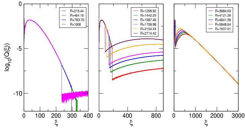
Figure 3: Plot as a function of \xi = mh of the logarithm of the probability, \log_{10} Q(\xi) , with Q(\xi) = \bar{Q}(\frac{\xi}{h}) , that the Kolmogorov scale is reached at scale m = \frac{\xi}{h} , for different Reynold's numbers and h = 10^{-3} \langle \xi \rangle .
