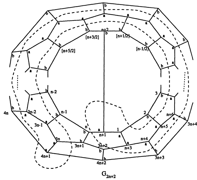
Fig. 2. The labelled graphs G_g
