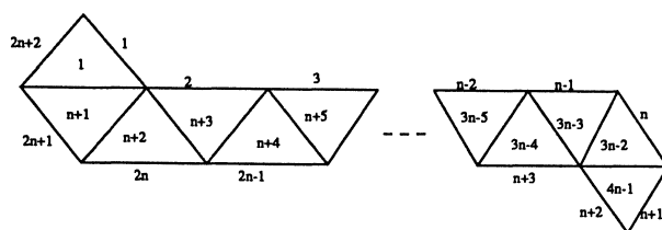
A subset, odd genus case g = 2n+1
