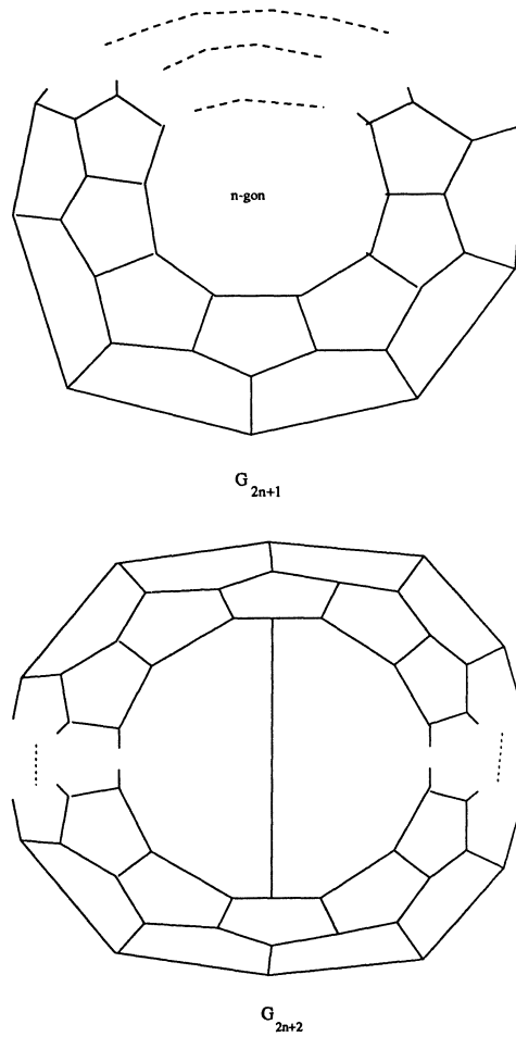
Fig. 1. The graphs G_g
