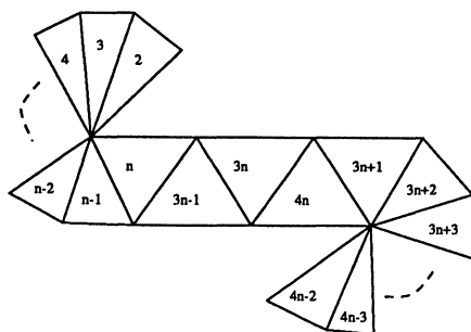
B subset, odd genus case g = 2n+1
