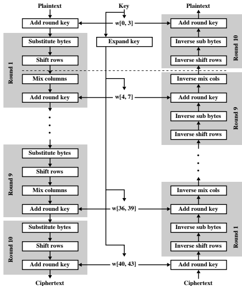
(a) Encryption
